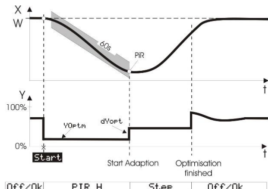
self-tuning [ \text{grad}(x)<0 ]
