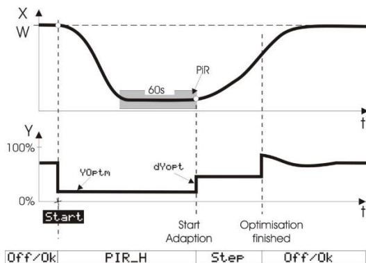
self-tuning [ \text{grad}(x)=0 ]
