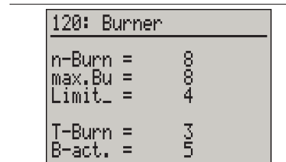
Fig. 7 Burner operating page:
