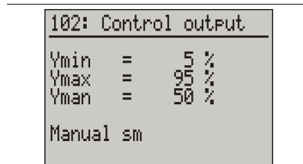
Fig. 6 Control signal operating page:
