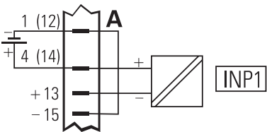
2-wire transmitter connection (e.g. INP1)
