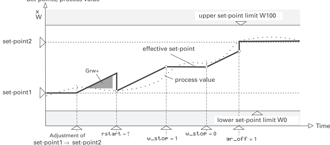
Fig.: 14 Effect of control inputs ( rstart , w-stop und sr_off ) on the set-point Set-points, process value
