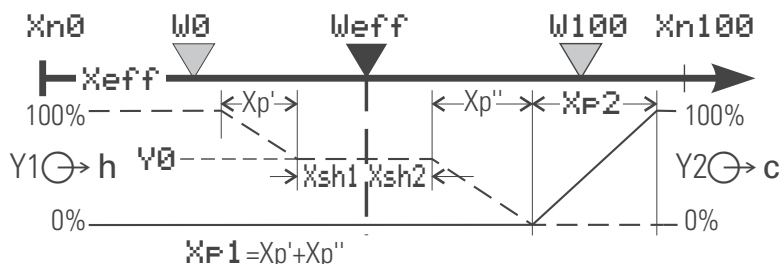
Fig.: 1 Static operating principle of a three-point controller
