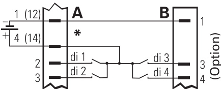
Energization of digital inputs (e.g. di1...di4)
