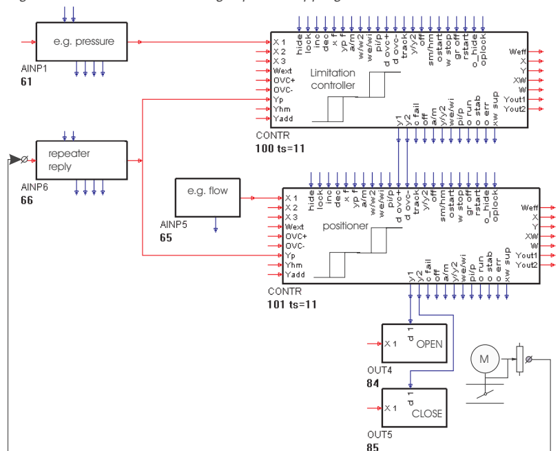
Fig.:23 Override control using 3-point stepping controllers
