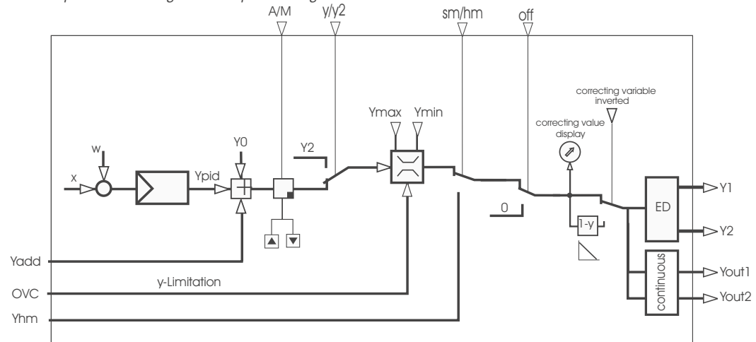
Fig.: 17 Steps of correcting variable processing
